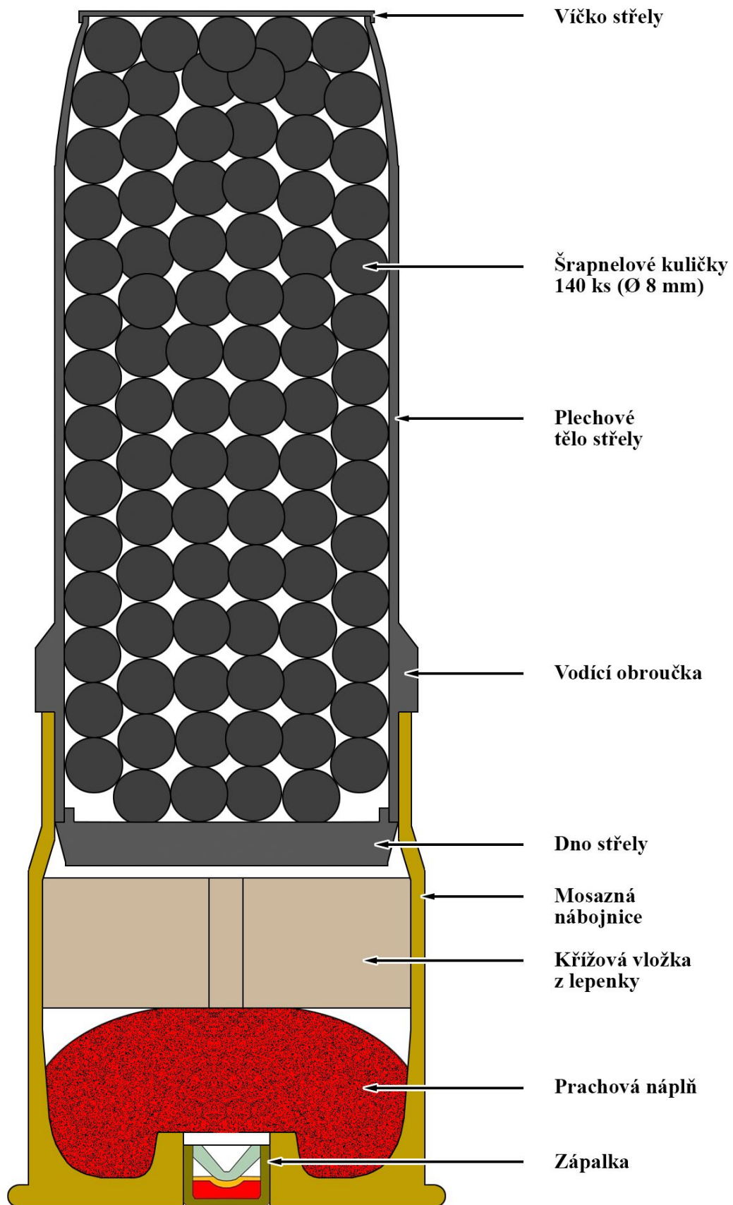
37 mm Bazooka model 2
